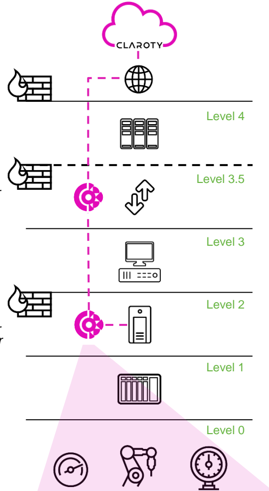
Example 3 tier deployment
